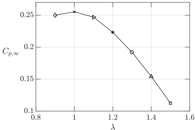
FIGURE 9. Reynolds number invariant power coefficient as a function of tip speed ratio. Symbols as in figure 8.
