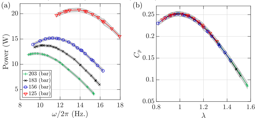
FIGURE 3. Power curves shown for a single Reynolds number of Re_D = 2.82 \times 10^6 at various tunnel conditions. Dimensional data is shown in physical units for plot (a) and then normalized with free-stream conditions for (b). Legend applies to both plots.
