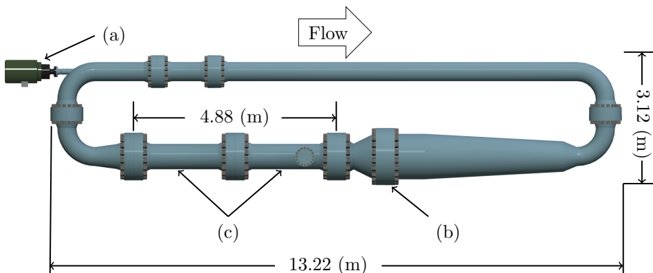
FIGURE 1. The High Reynolds number Test Facility or HRTF located at the Princeton Gas Dynamics Laboratory. The external motor (a) drives an internal impeller pump which moves compressed air through the return section and on to the flow conditioning and contraction at (b) where it next enters the two working sections at (c). The facility is designed to produce laminar slug flow inside the test section at low turbulence levels.
