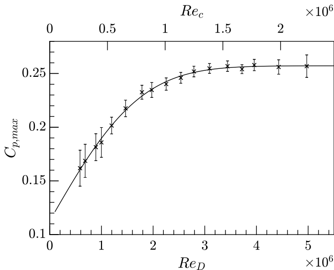
FIGURE 7. The maximum measured power coefficient shown as a function of Reynolds number based on diameter. Top axis is given in terms of the local blade conditions and taking \lambda = 1 . The ‘x’ symbols are measured data, and the solid line is a fitted error function given by equation 3.1.
