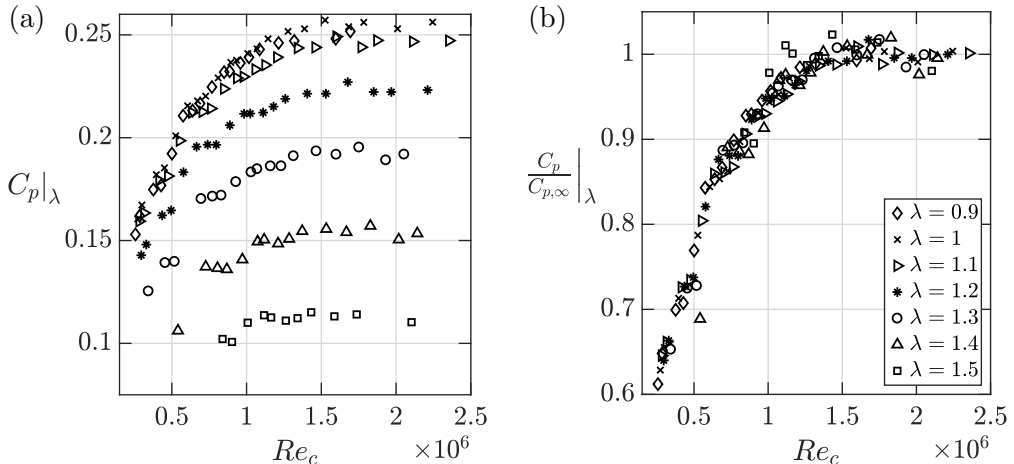
FIGURE 8. Power coefficient shown as a function of the blade Reynolds number in (a). Data has been interpolated to a fixed \lambda grid as given by the legend of (b). Subfigure (b) gives this same data normalized by the Reynolds number invariant value of C_p , found as the mean power coefficient for cases where Re_c > 1.5 \times 10^6 . Legend applies to both plots.
