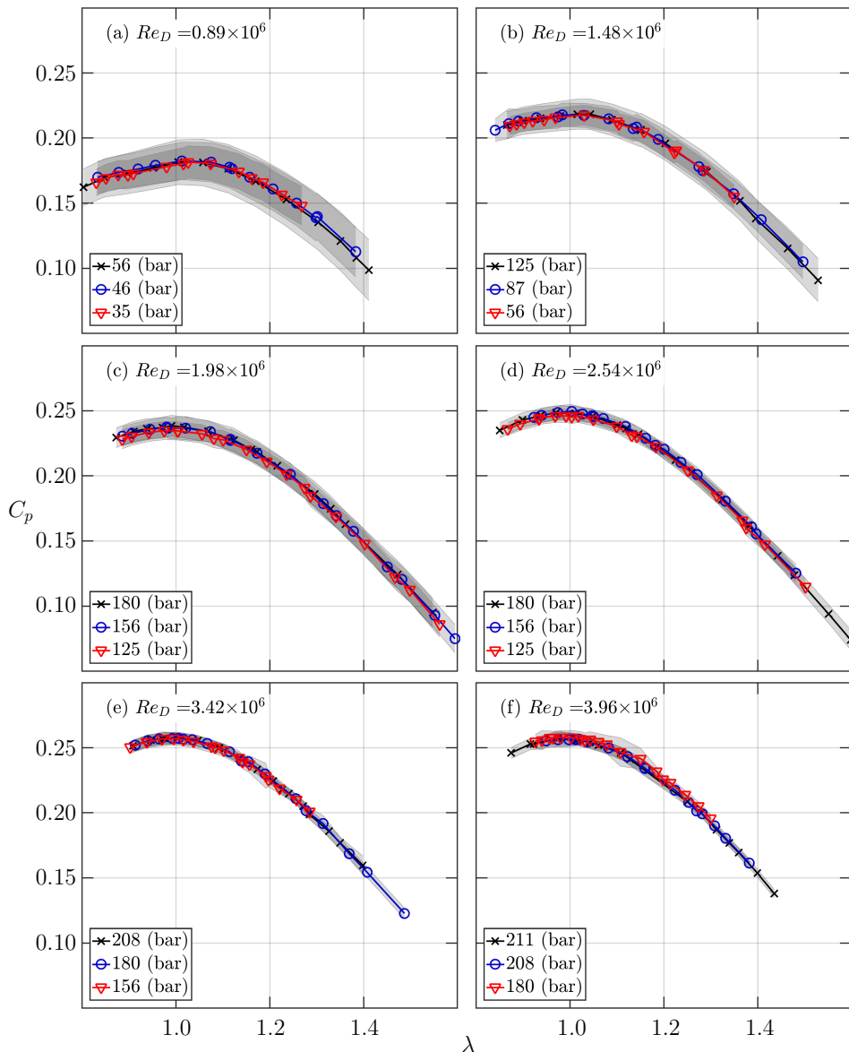
FIGURE 4. Collapse of data as Reynolds number increases (from (a) to (f)). Data is shown referenced to the tunnel static pressure for convenience (actual density and viscosity calculated at each run condition from measured pressure and temperature).
