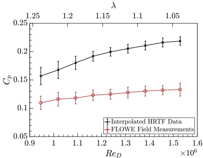
FIGURE 6. Power coefficient as a function of Reynolds number based on diameter and tip speed ratio. HRTF data (black ‘x’) has been interpolated onto the average operating tip speed ratios for the FLOWE wind turbine (red ‘o’).
