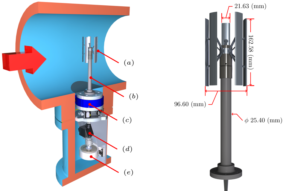
FIGURE 2. Rendering of VAWT model inside cut-away of HRTF test section. Labels correspond to (a) 5 bladed VAWT model, (b) tower housing, (c) six-component force/moment sensor, (d) torque transducer with speed encoder, and (e) magnetic hysteresis brake for speed control. Red arrow gives direction of flow. Detail view of VAWT model is shown with dimensions at right.
