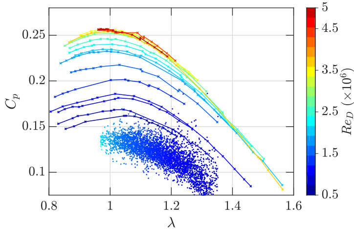
FIGURE 5. The power coefficient plotted as a function of tip speed ratio and Reynolds number (given by colorbar). HRTF data is given by cross-hatch marks while FLOWE field data is shown as a point cloud.
