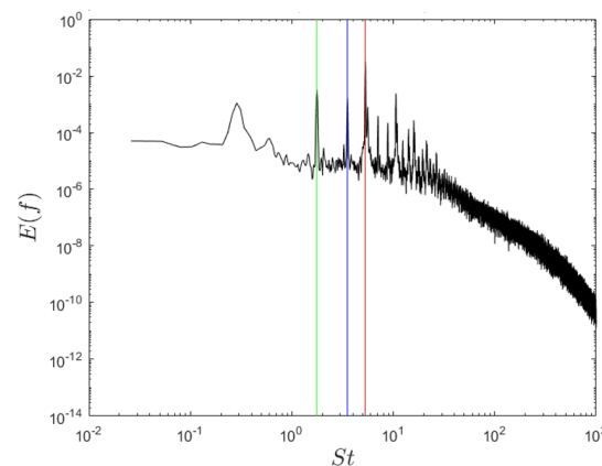
Figure 9. Power spectral density at Re_D=2.7 \times 10^6 for x/D=0.77 and r/D=0.526 . Each colored line represents a different harmonic with respect to the turbine's rotation rate up to the third harmonic.
